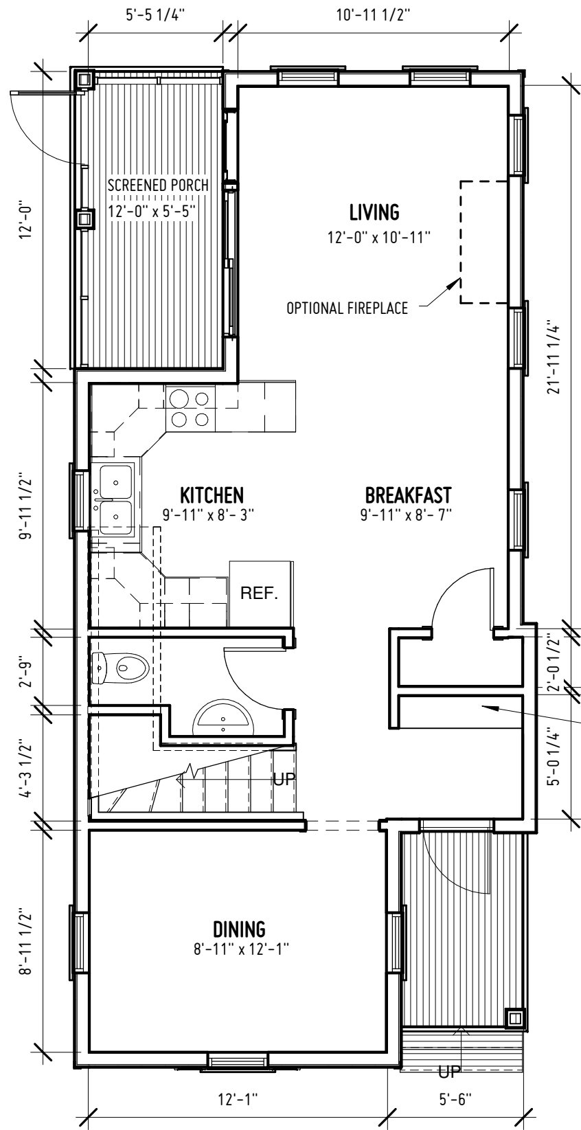
FIRST FLOOR HEATED SF: 611 SF
