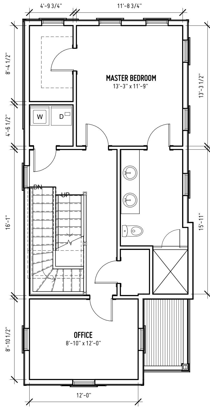
SECOND FLOOR HEATED SF: 688 SF
