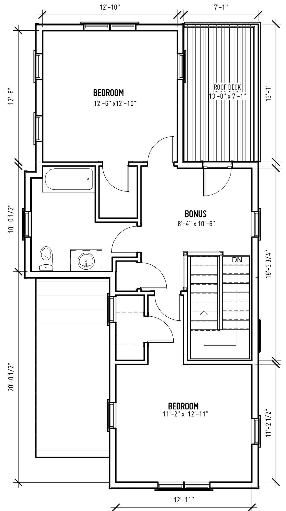
THIRD FLOOR HEATED SF: 704 SF
