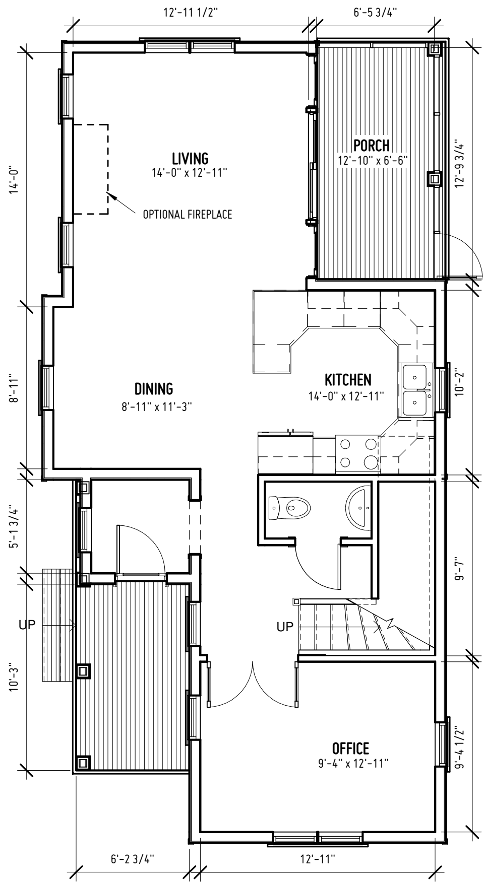
FIRST FLOOR HEATED SF: 737 SF
