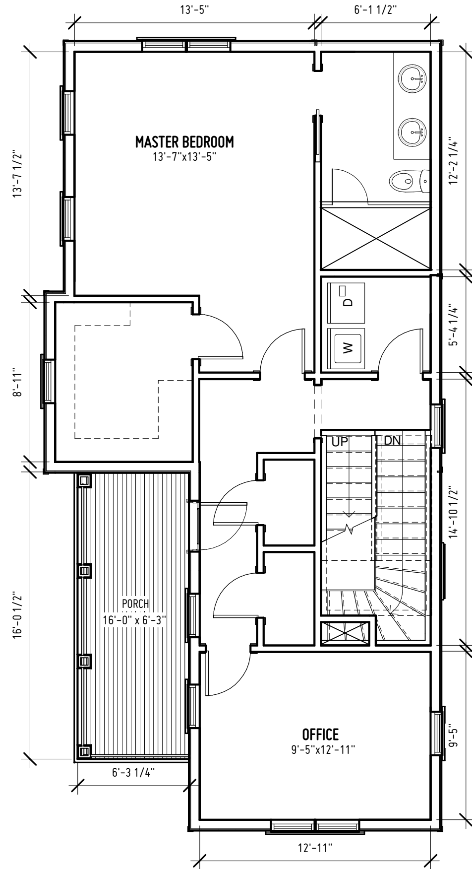
SECOND FLOOR HEATED SF: 802 SF
